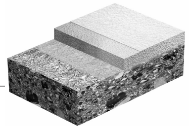
Self-Levelling/Broadcast Surfacing
