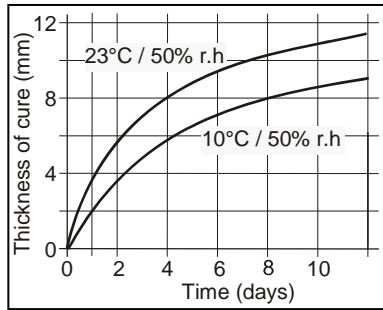
Diagram 1: Curing speed for Sikaflex®-296
