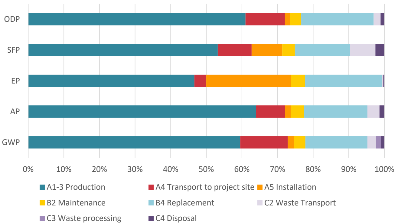
Figure 4: Relative contribution of life cycle modules to potential environmental impacts for 1 m² of Sikafloor® NA Ucrete® (average coverage, 20-yr industrial market service life) 3
