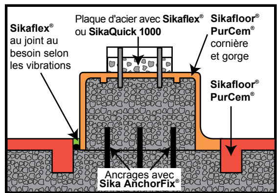
Sikafloor® PurCem® – Socle de machine
