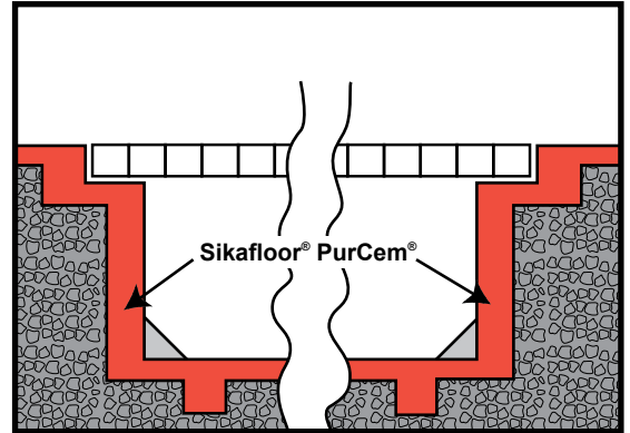
Sikafloor® PurCem® – Rigole recouverte
