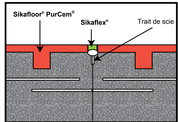
Sikafloor® PurCem® – Joint au sol
