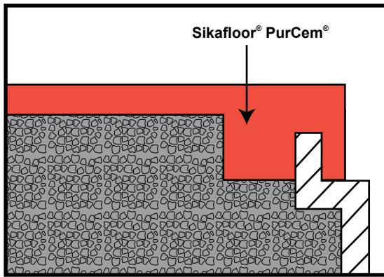
Sikafloor® PurCem® – Glazed drain edge detail
