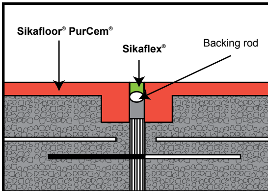
Sikafloor® PurCem® – Expansion joint
