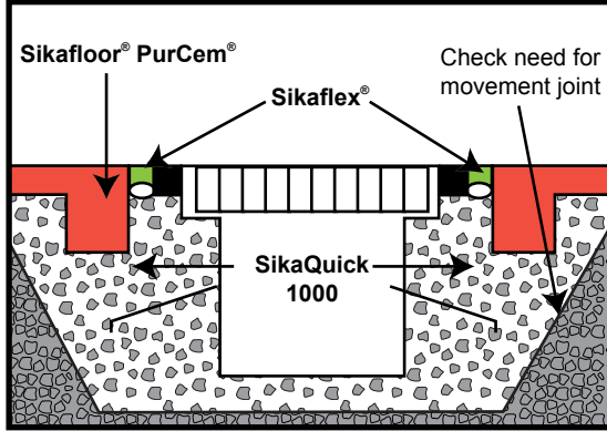
Sikafloor® PurCem® – Glazed drain edge detail
