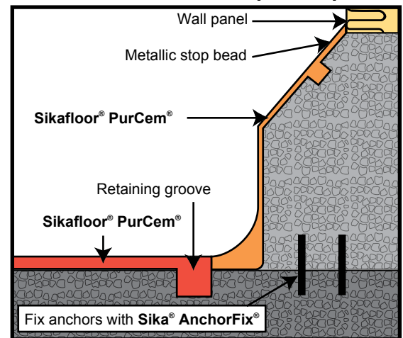
Sikafloor® PurCem® – Bumper / curp detail
