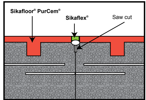
Sikafloor® PurCem® – Induced floor joint
