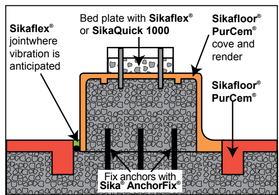
Sikafloor® PurCem® – Machine base
