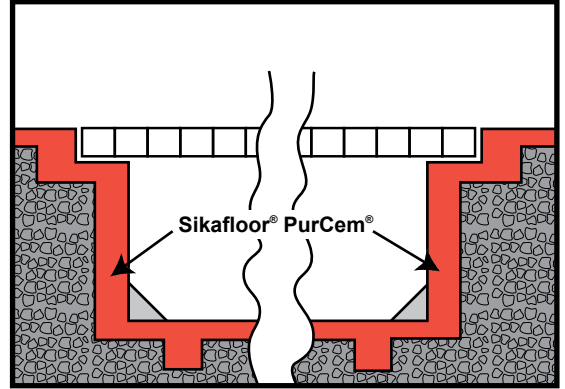
Sikafloor® PurCem® – Lined trench
