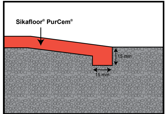
Sikafloor® PurCem® – “Keyed” edge detail
