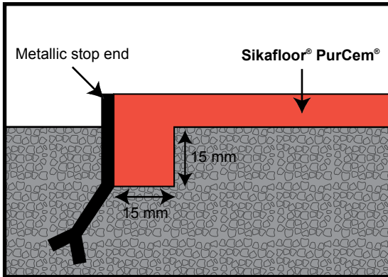
Sikafloor® PurCem® – Metallic stop end
