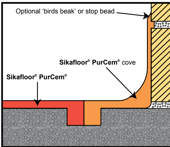
Sikafloor® PurCem® – Floor to wall cove
